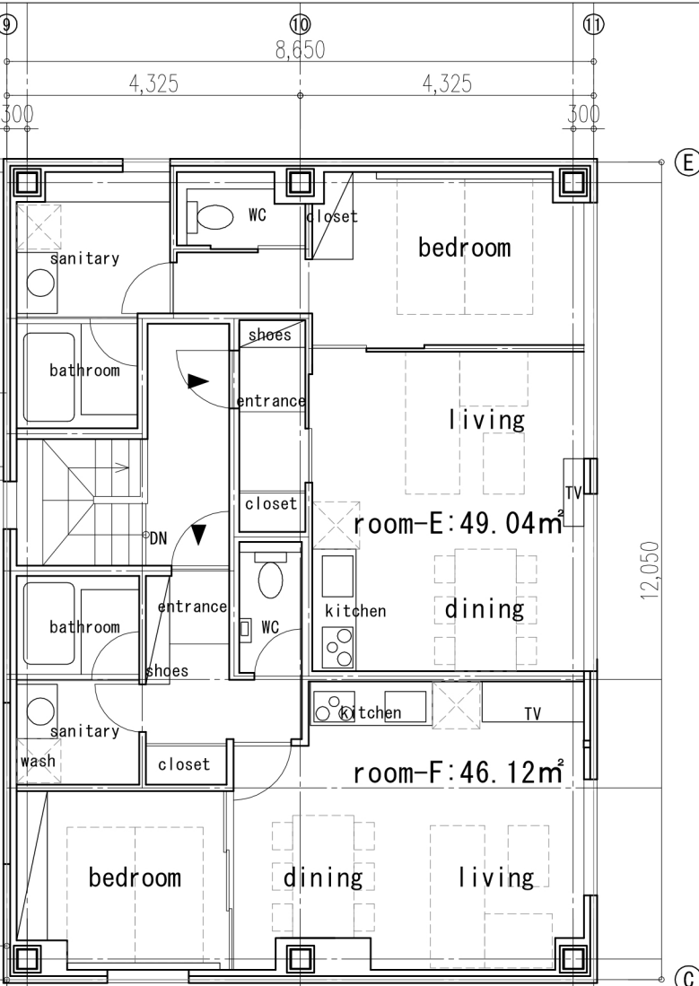
<3F plan>
