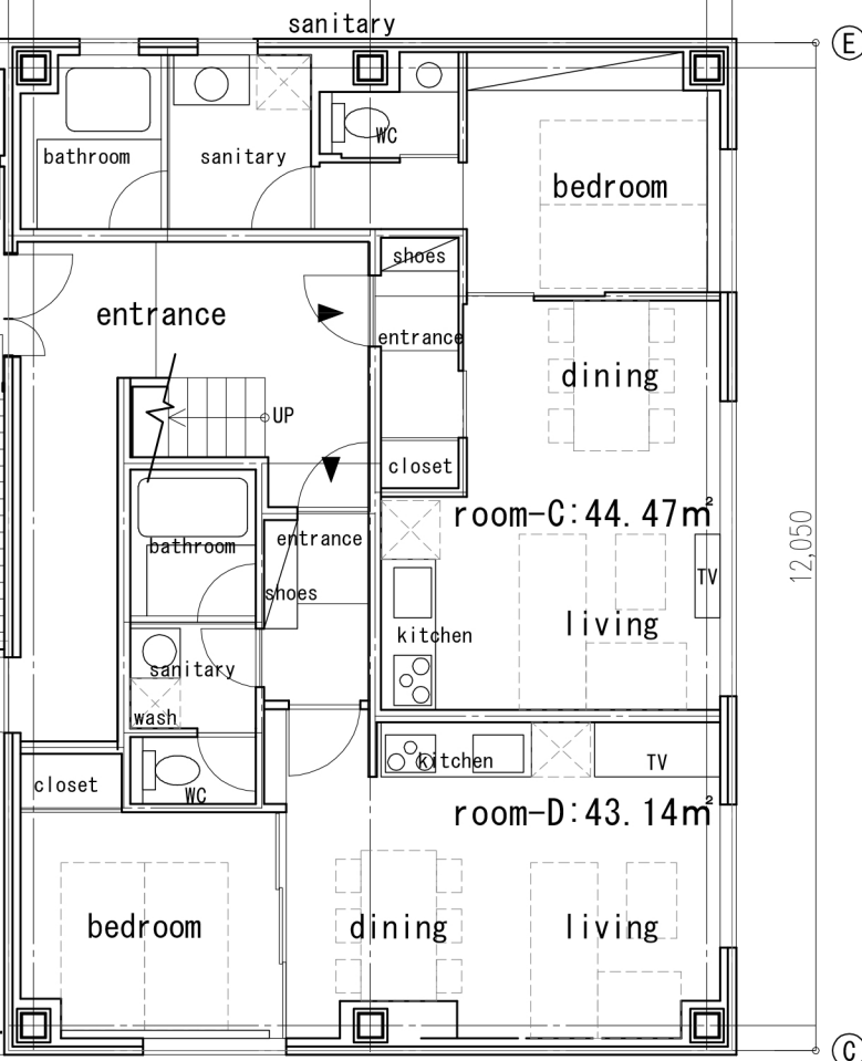
<2F plan>
